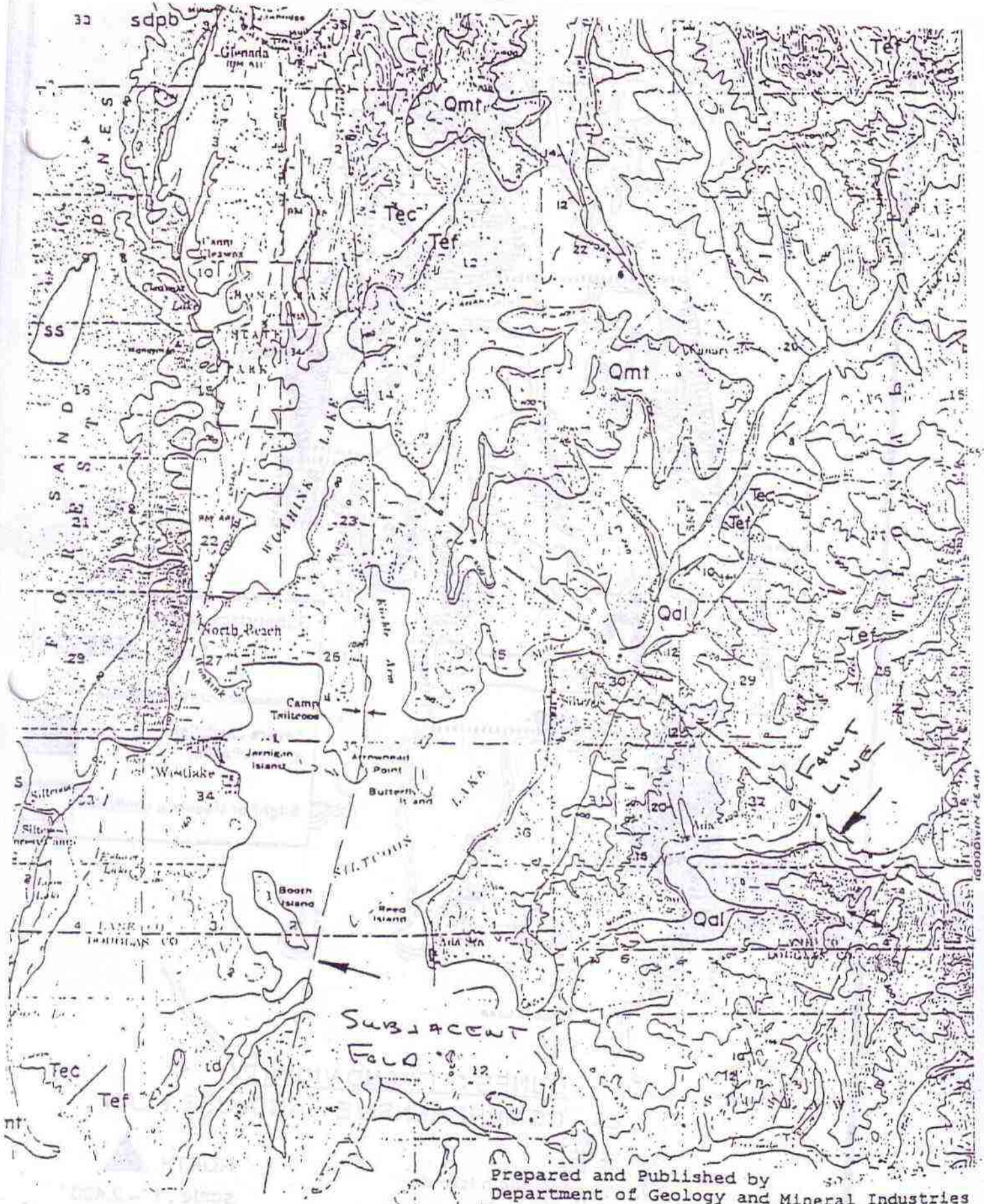
APPENDIX J - (Earthquake Faults)
